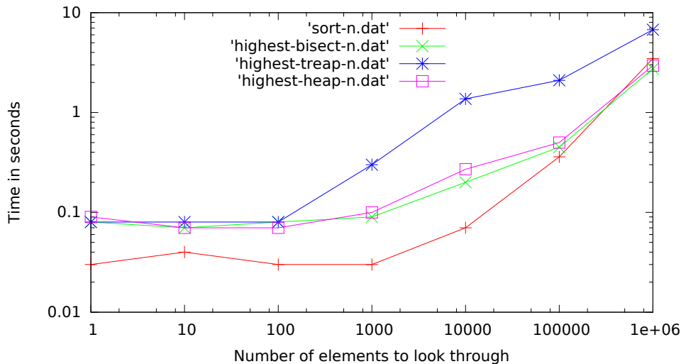
Inspect n values, keep m: n varied, m is 1000
