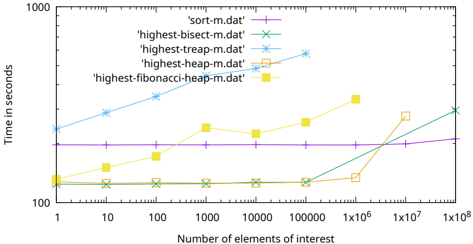
Inspect n values, keep m: m varied, n is a bit under 500,000
