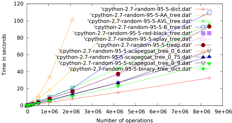
cpython-2.7, random, 95% get, 5% set.pdf
