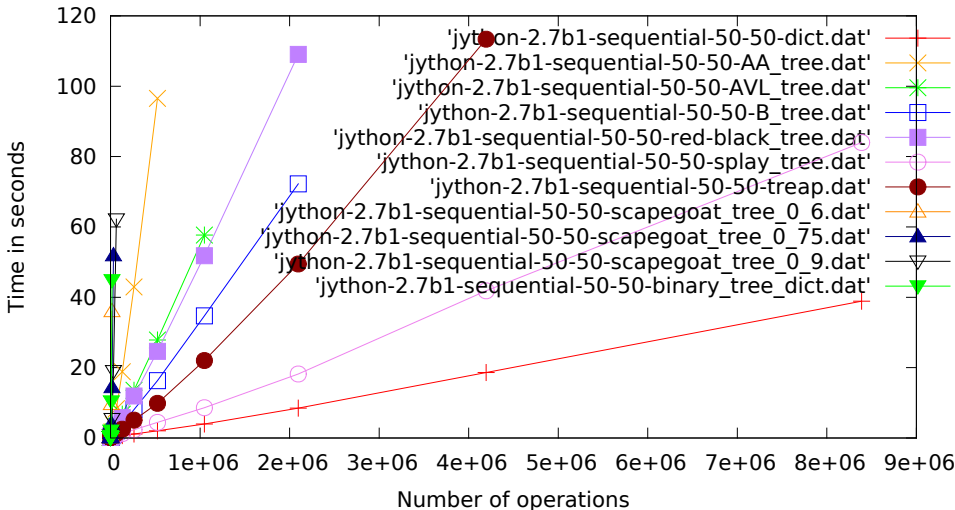
jython-2.7b1, sequential, 50% get, 50% set.pdf
