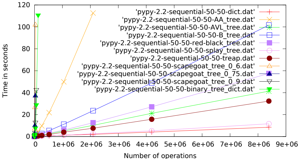
pypy-2.2, sequential, 50% get, 50% set.pdf
