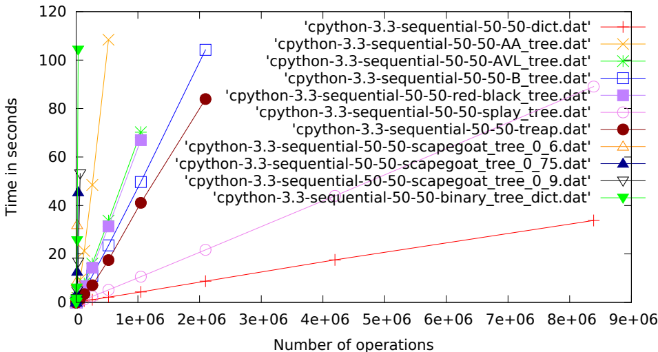
cpython-3.3, sequential, 50% get, 50% set.pdf
