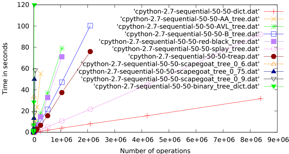
cpython-2.7, sequential, 50% get, 50% set.pdf
