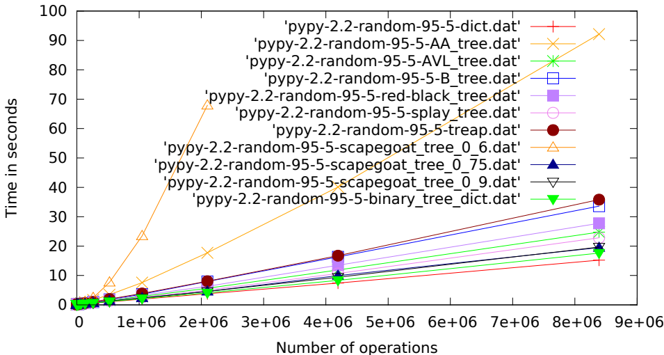
pypy-2.2, random, 95% get, 5% set.pdf
