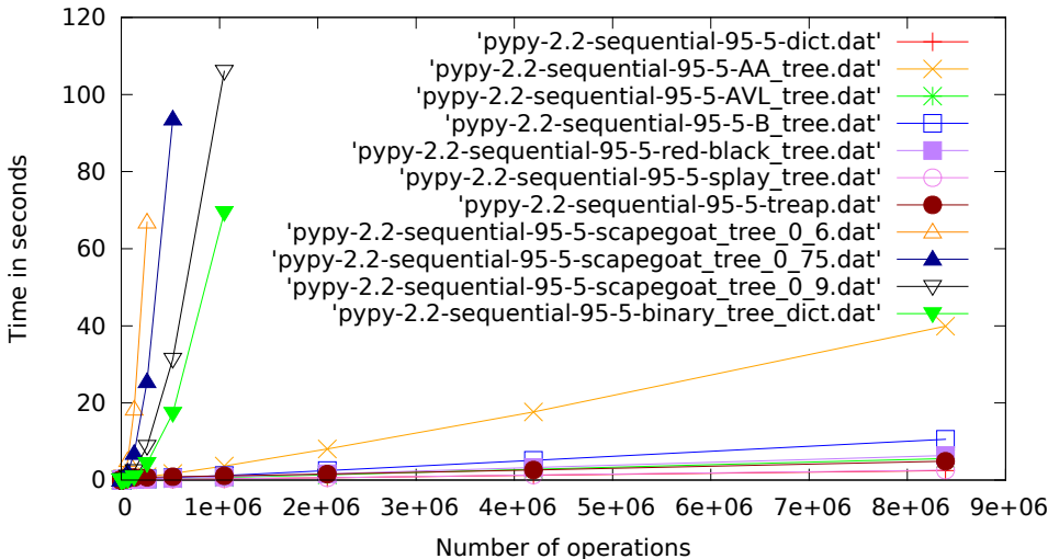
pypy-2.2, sequential, 95% get, 5% set.pdf
