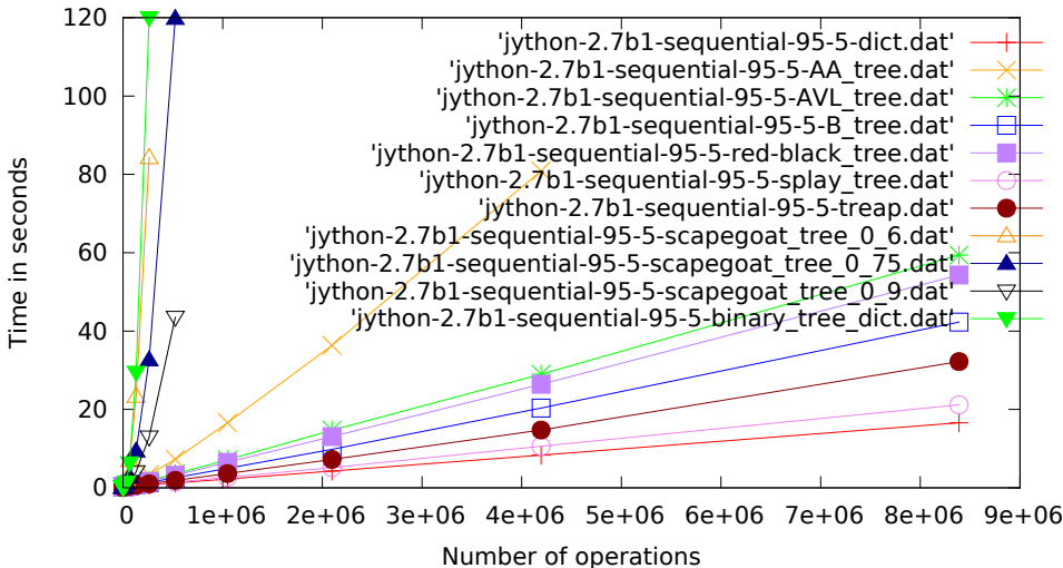
jython-2.7b1, sequential, 95% get, 5% set.pdf
