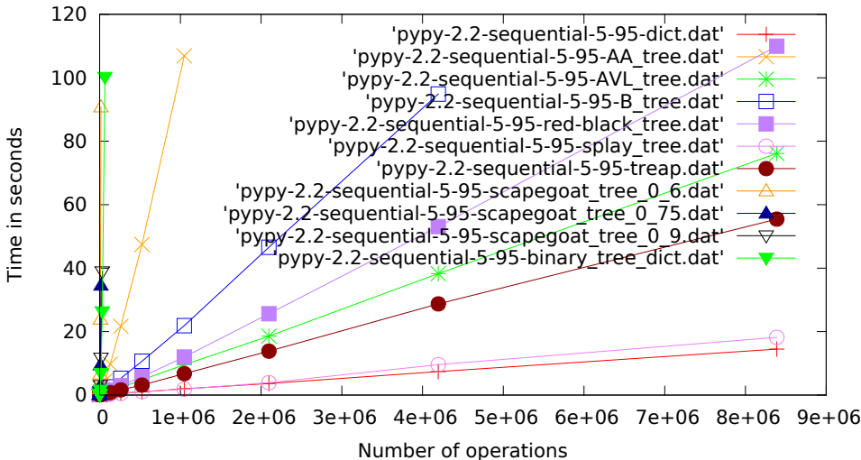
pypy-2.2, sequential, 5% get, 95% set.pdf
