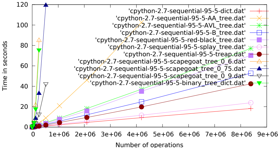
cpython-2.7, sequential, 95% get, 5% set.pdf
