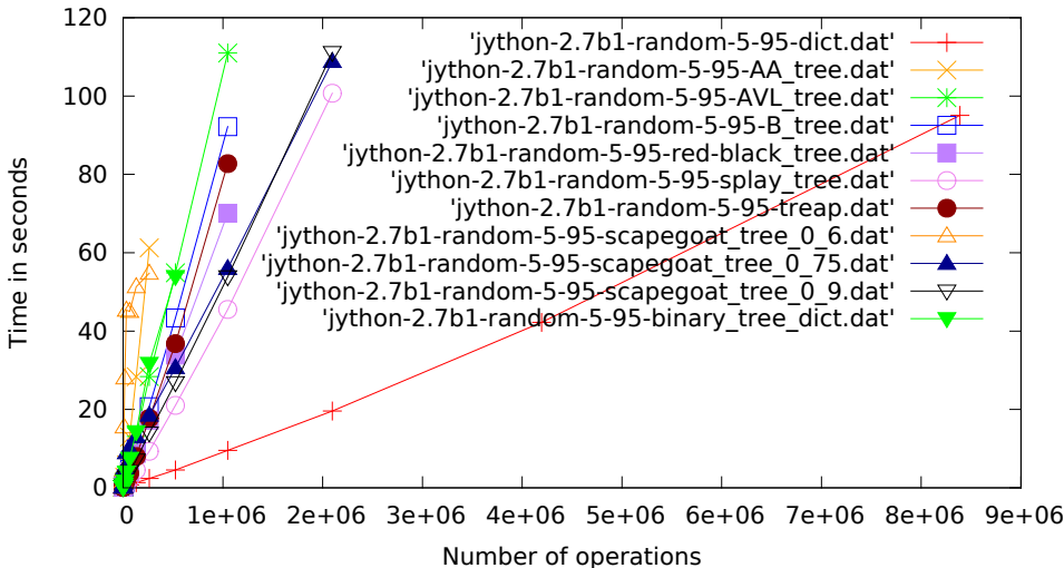
jython-2.7b1, random, 5% get, 95% set.pdf
