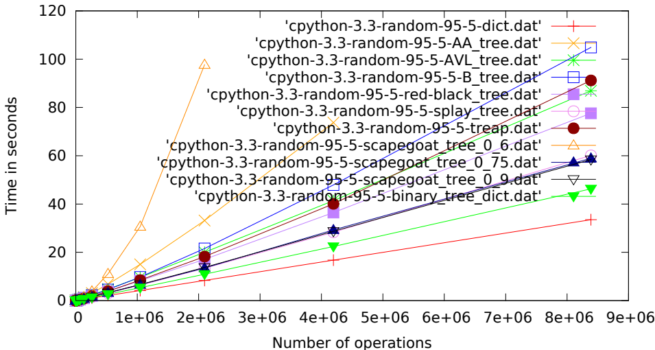
cpython-3.3, random, 95% get, 5% set.pdf
