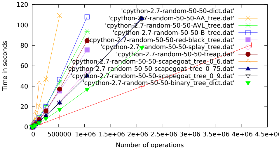
cpython-2.7, random, 50% get, 50% set.pdf
