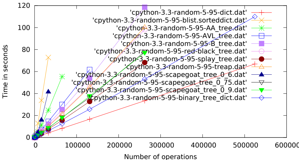
cpython-3.3, random, 5% get, 95% set.pdf
