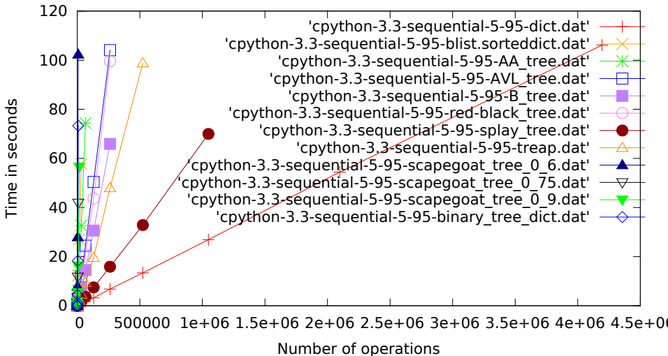
cpython-3.3, sequential, 5% get, 95% set.pdf
