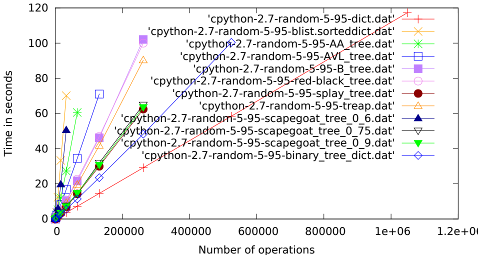
cpython-2.7, random, 5% get, 95% set.pdf
