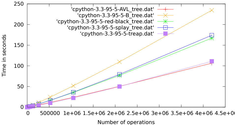
cpython-3.3, 95% get, 5% set.pdf
