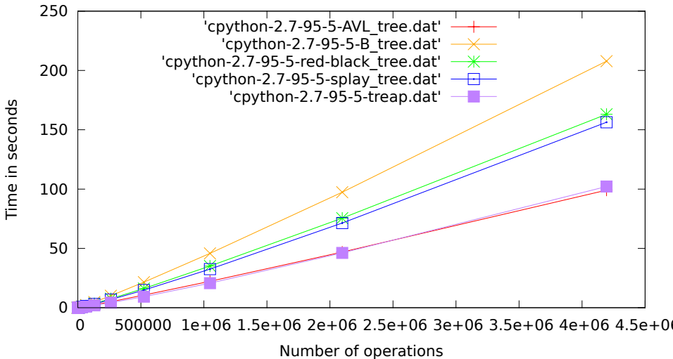
cpython-2.7, 95% get, 5% set.pdf
