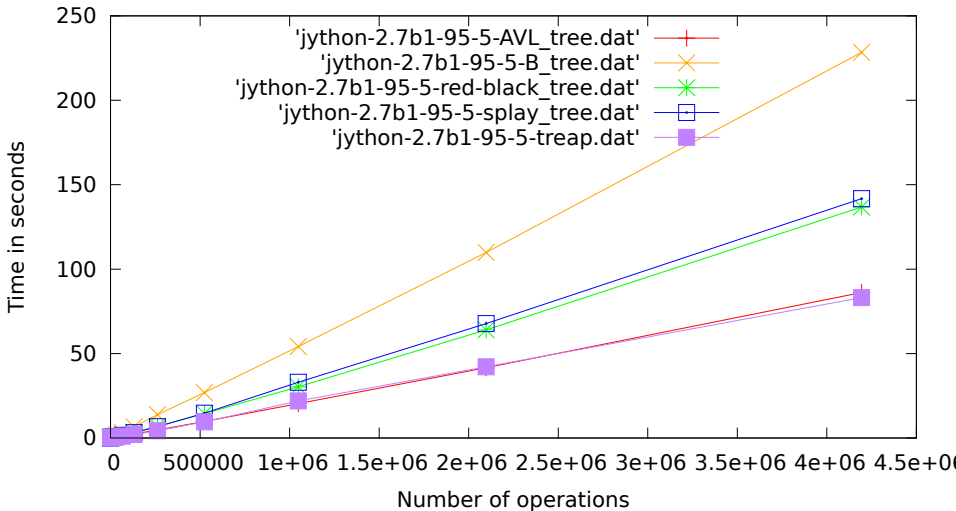
jython-2.7b1, 95% get, 5% set.pdf
