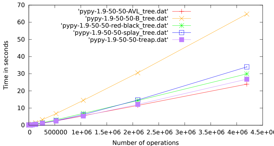
pypy-1.9, 50% get, 50% set.pdf
