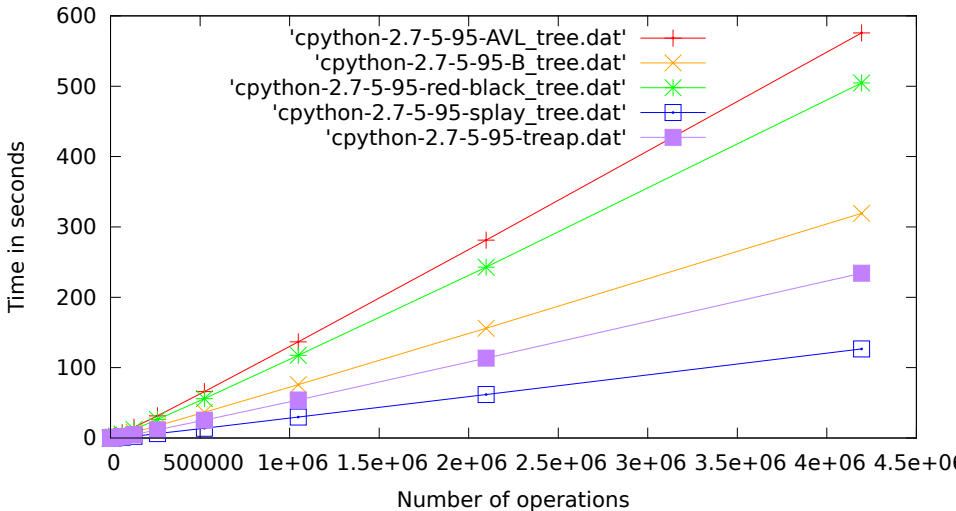
cpython-2.7, 5% get, 95% set.pdf
