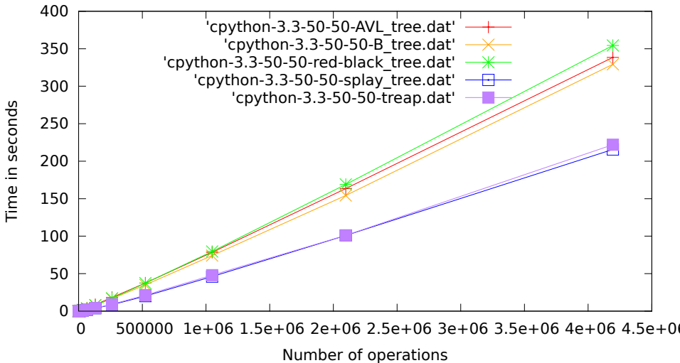
cpython-3.3, 50% get, 50% set.pdf
