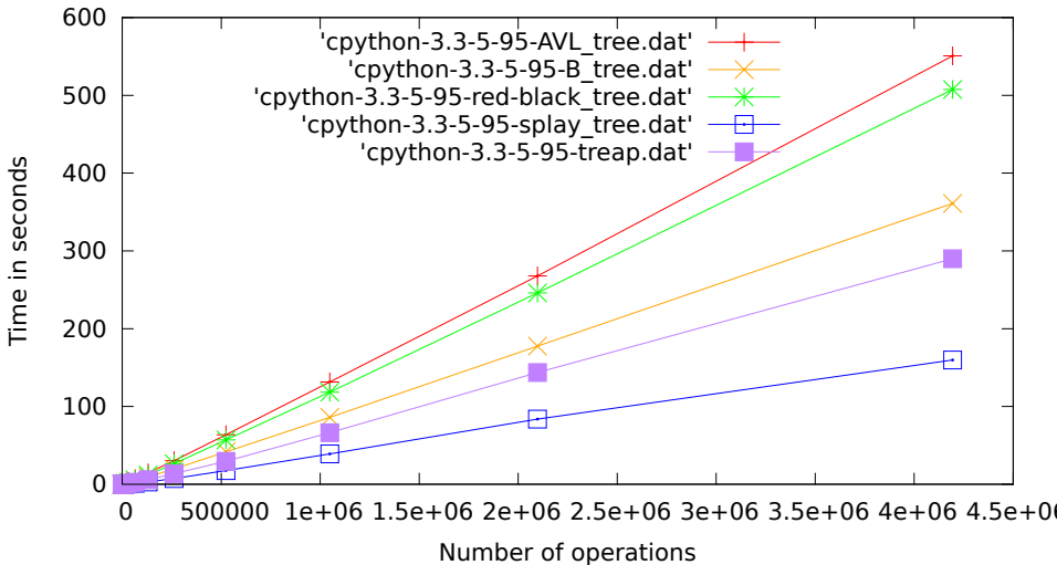
cpython-3.3, 5% get, 95% set.pdf
