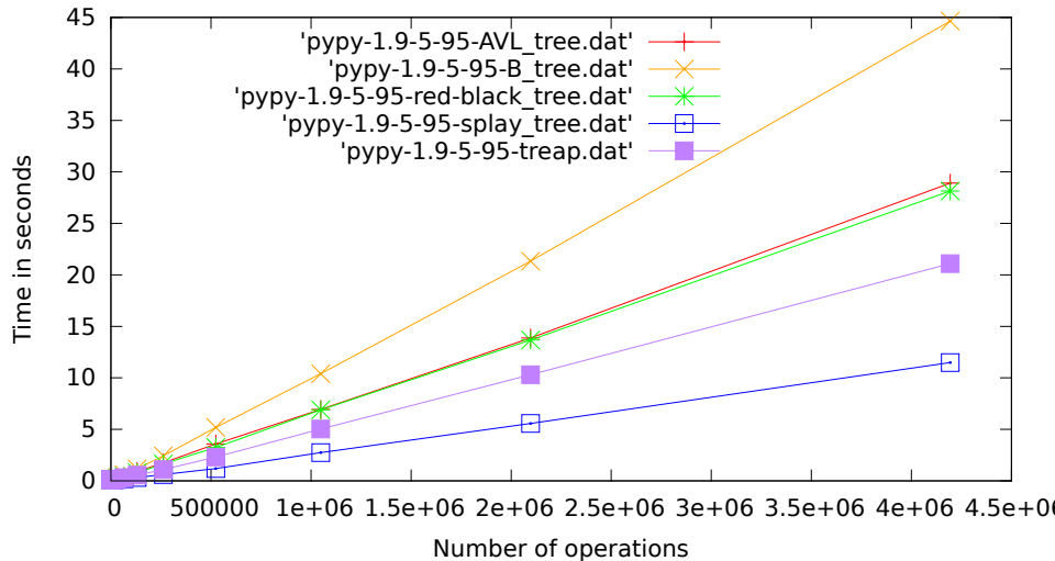
pypy-1.9, 5% get, 95% set.pdf
