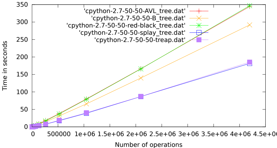
cpython-2.7, 50% get, 50% set.pdf
