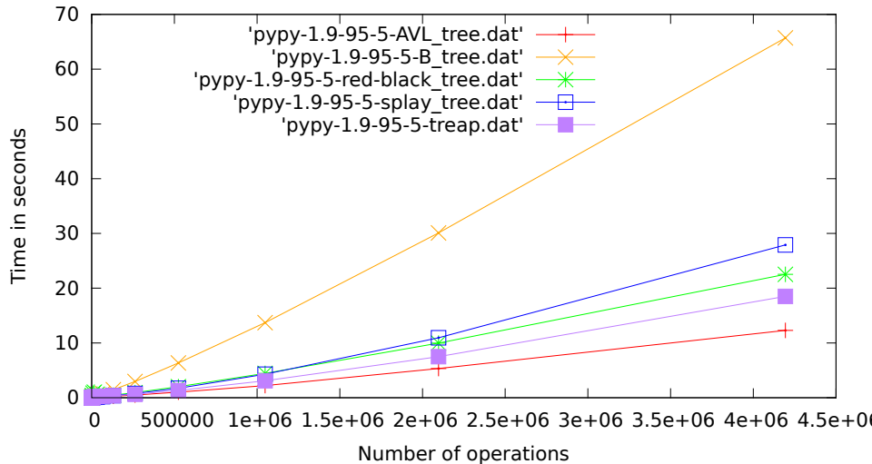
pypy-1.9, 95% get, 5% set.pdf
