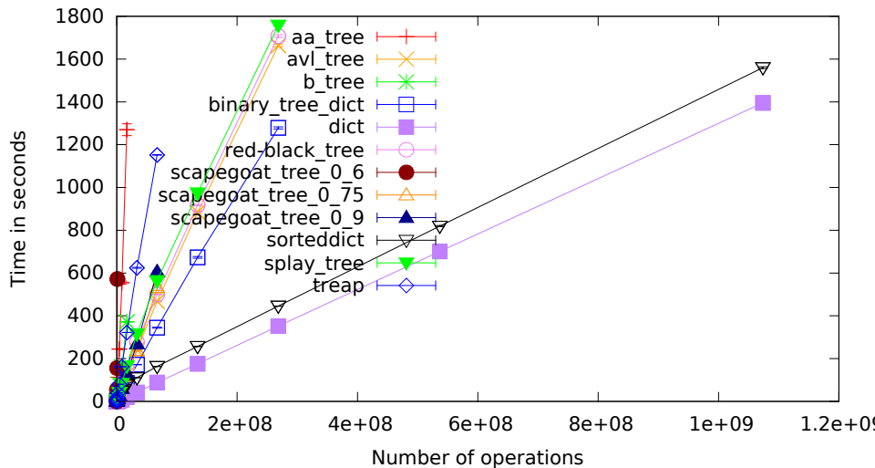
pypy-2.5.0, random.pdf
