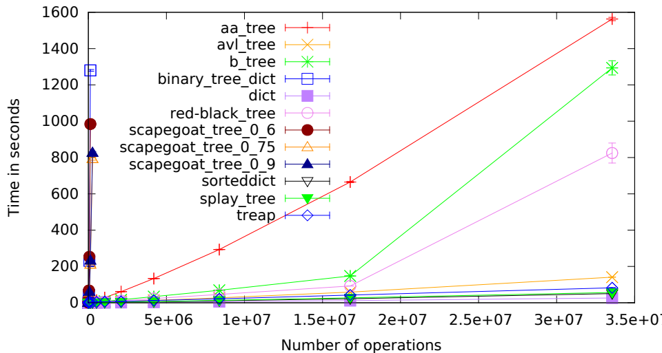
pypy3-2.4.0, sequential.pdf
