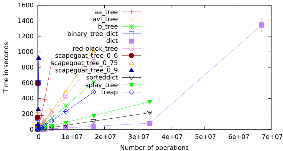
cpython-3.4, sequential.pdf
