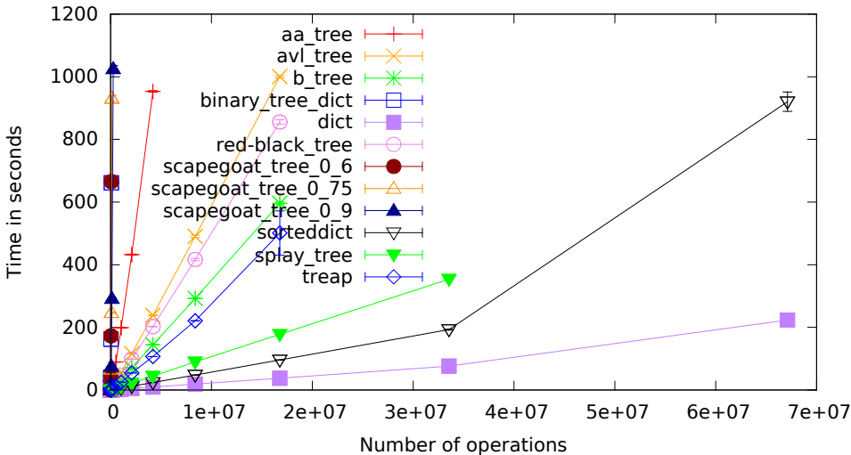
cpython-2.7, sequential.pdf
